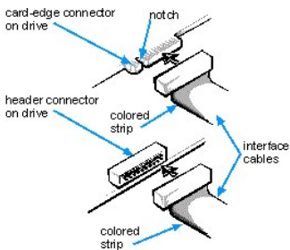
Figure 5. Drive Interface Connectors
