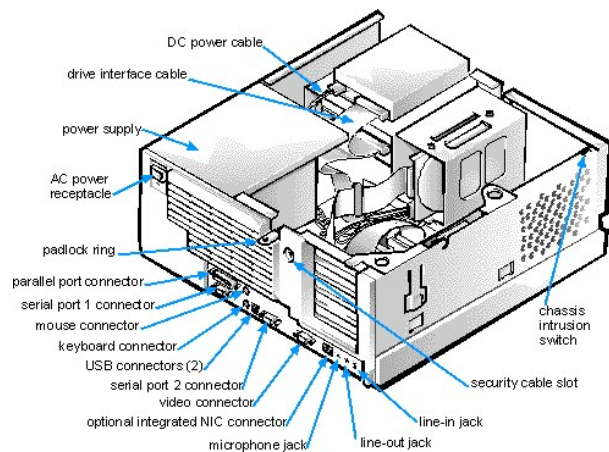
Figure 5. Inside the Chassis
