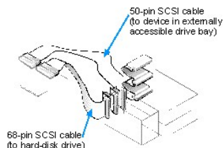
Figure 13. Internal SCSI Cables
