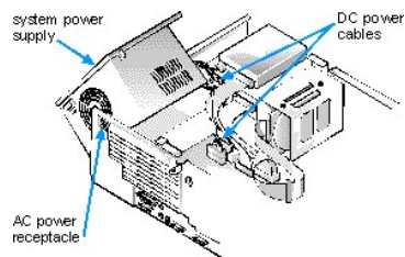
Figure 8. Rotating the Power Supply
