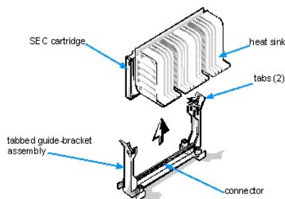
Figure 10. Removing the Microprocessor
