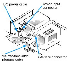
Figure 9. Attaching Diskette Drive or Tape Drive and DC Power Cables
