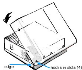
Figure 3. Replacing the Computer Cover
