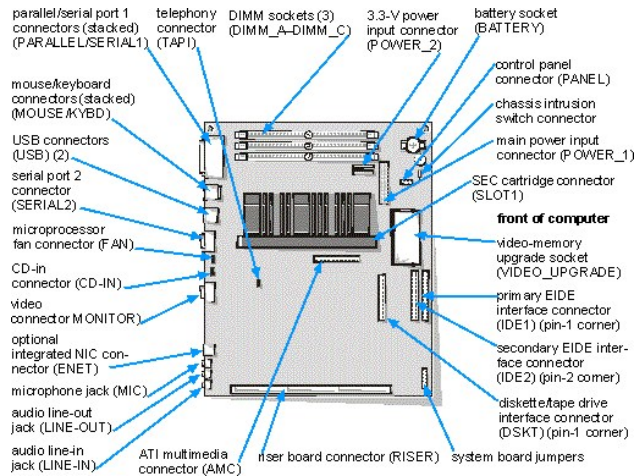
Figure 1. System Board Features
