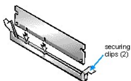
Figure 7. Installing a DIMM
