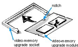
Figure 9. Installing a Video-Memory Upgrade Module
