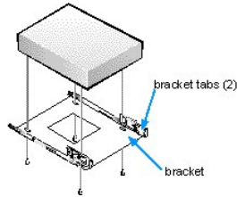
Figure 7. Attaching the Drive Bracket to the New Drive
