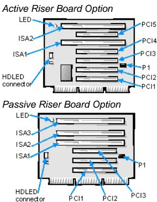
Figure 3. Riser Board Expansion-Card Connectors
