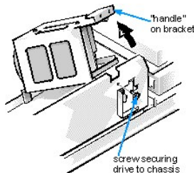
Figure 10. Removing the Hard-Disk Drive Bracket
